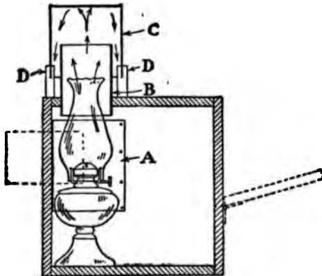
FIG. 342. — Cross-section of Reflectoscope.
